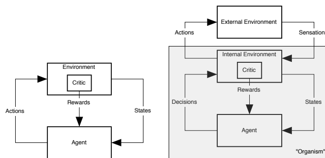
Figure 1: Agent-environment interactions in reinforcement learning; adapted from Barto et al. (2004). See text for discussion.
